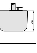
Wc monoblocco Brio con cassetta Wc monoblock Brio with cistern Bidet Brio a terra Bidet Brio back to wall
